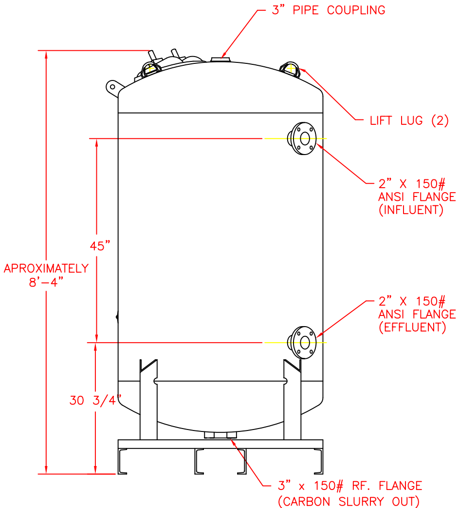
ELEVATION / FRONT VIEW
